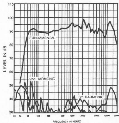
FIGURE 3 Interface 2 Frequency Response (1 watt at 1 meter)
