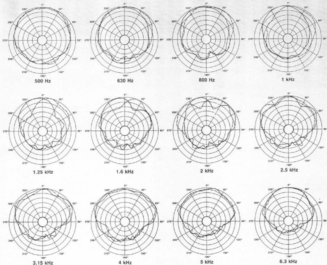
FIGURE 1 Interface 2 Polar Response
